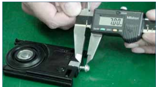
Tightening at fixed height.
